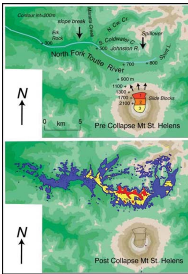
Figure 3. Top panel: Mount Saint Helens vicinity. Colours and labels indicate the three slide blocks that initially accelerated northwards towards Johnston Ridge. Bottom panel: deposit distribution and thickness as measured by pre- and post-DEMs (contours 10, 50 and 90 m). Note decrease in thickness at slope break.
