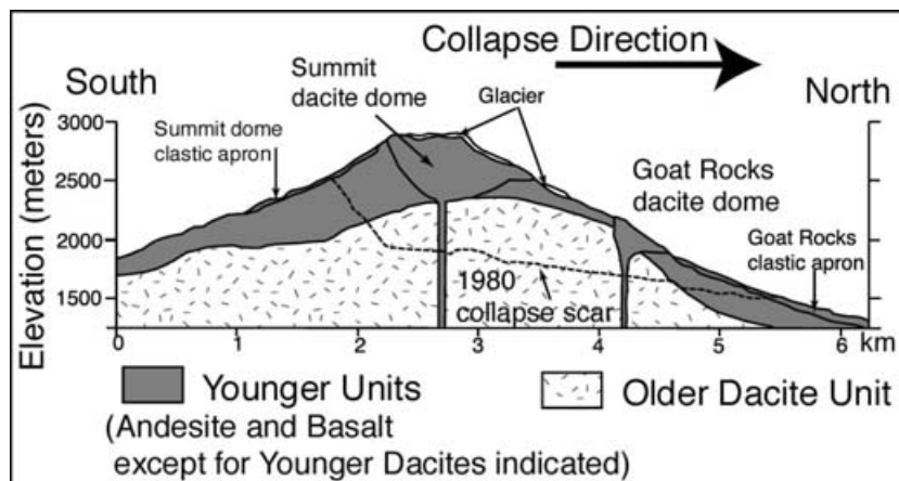
Figure 2. Simplified north–south cross-section of pre-collapse Mount Saint Helens along the axis of the collapse structure: modified after Glicken (1996). Geology of the pre-collapse Mount Saint Helens is dominated by the upper Andesite–Basalt unit and the lower Older–Dacite Unit.
