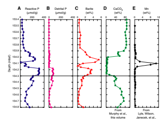
F3. Geochemical components vs. depth, p. 18.
