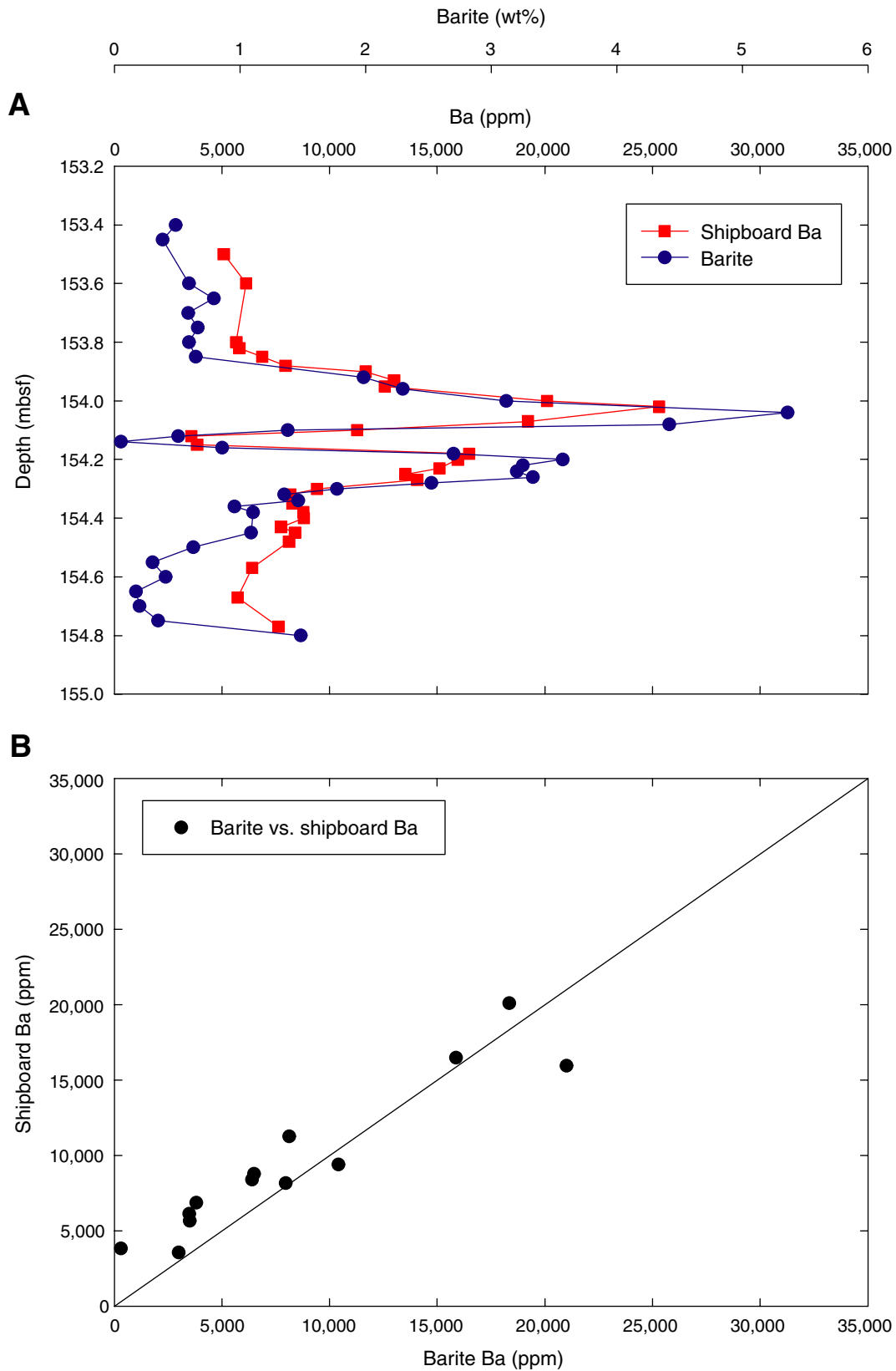
Figure F2. A. Barite (Table T1, p. 20) and shipboard Ba (Table T3, p. 22) (Lyle, Wilson, Janecek, et al., 2002) vs. depth. B. Barite vs. shipboard Ba. Only the samples to which depth horizons exactly correspond are plotted. For linear regression, slope = 0.75 \pm 0.08 and y-intercept = 3300 \pm 800 ; r^2 = 0.89 .
