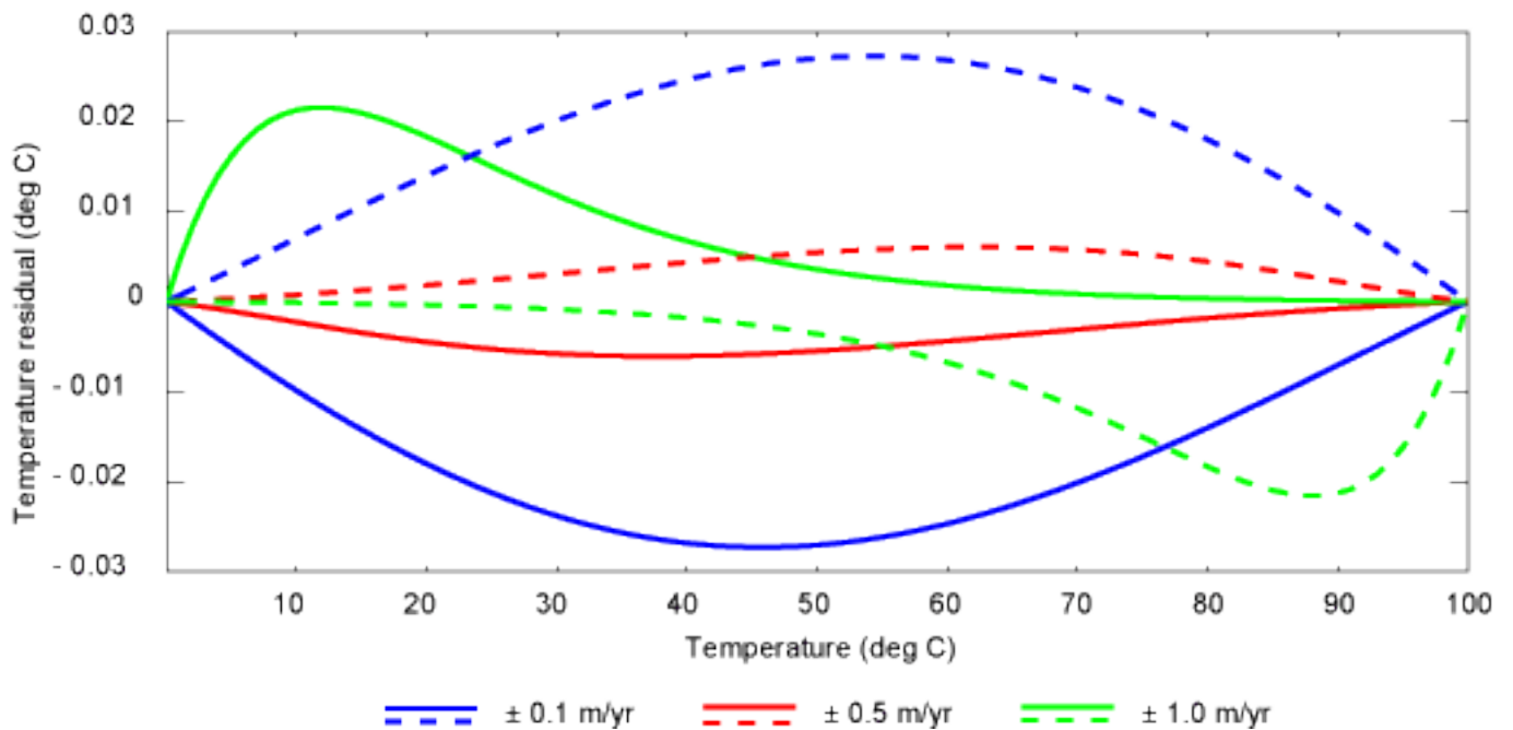
A. Comparison with analytical solutions at seven discrete seepage rates
