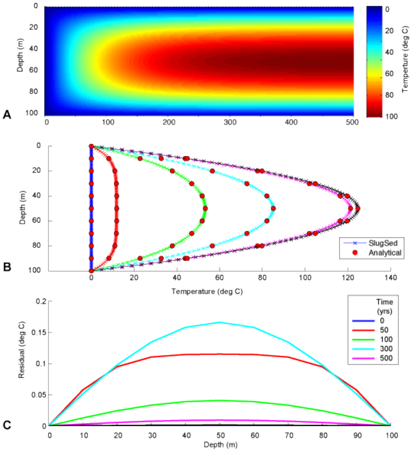
A. Temperature as a function of time within the slab B. Comparison with analytical solutions at five discrete times C. Residuals
